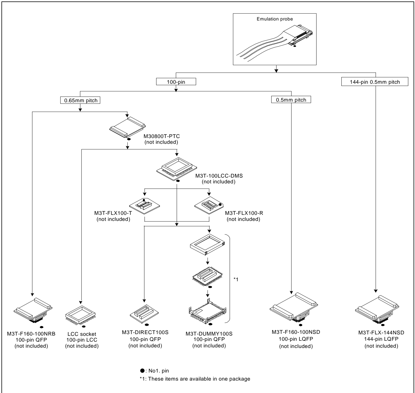
Figure 2.7 Connection of the M30850T2-EPB and user system
